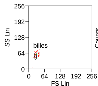
Cyan URP 2014-06-17
