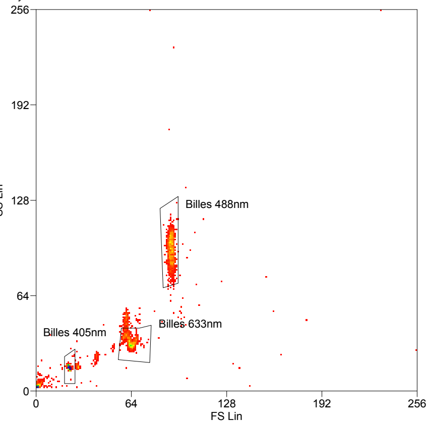
Cyan FlowCheck 2017-09-25
